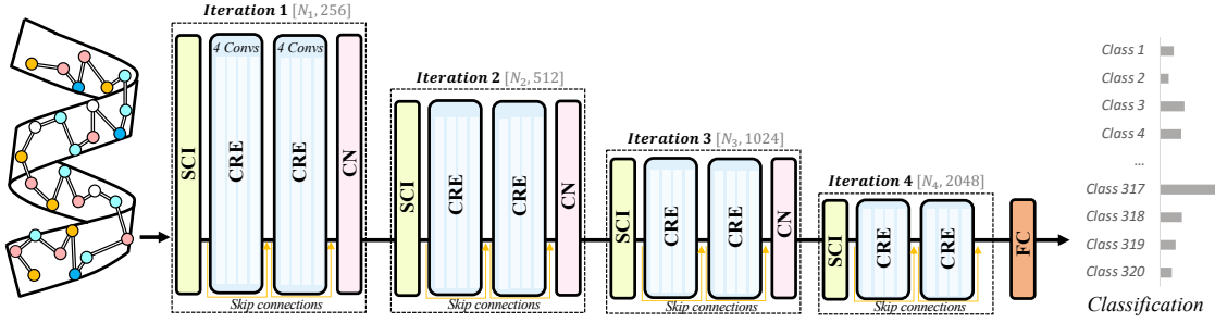
Figure 2. Our neural clustering framework architecture with four iterations. Given a protein, a set of 1D and 3D amino acids, our method adopts an iterative clustering algorithm to explore the most representative amino acids. At each iteration, B cluster representation extraction blocks are utilized to extract cluster features. The clustering nomination operation selects the fraction \omega of amino acids for the next iteration, that N_t = \lfloor \omega \cdot N_{t-1} \rfloor . Details of the framework can be seen in §3.3.
