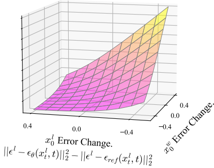
Figure 2. Loss surface visualization. Loss can be decreased by improving at denoising x_0^l and worsening for x_0^w . A larger \beta increases surface curvature.
