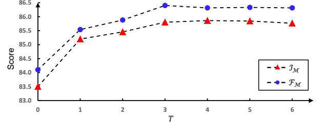
Figure 7. Comparison of performance characteristics with the number of iterations T on the DAVIS-16 [20] dataset.
