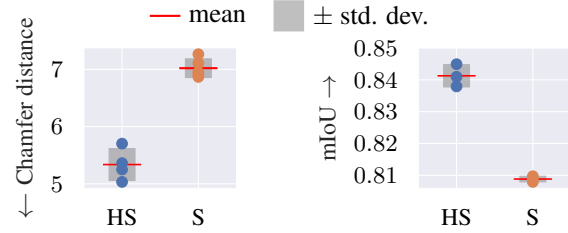
Figure 2. Chamfer distance (lower is better) and mIoU (higher is better) for HEAL-SWIN (HS) and SWIN (S). Details are provided in Section 4.3 and in Section 4.1.2.
