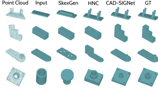
Figure 5. Visual results for auto-completion from user input on DeepCAD [42] dataset. From left to right, input point cloud, CAD model reconstruction from user input CAD sequence, SkexGen [44], HNC [45], CAD-SIGNet (ours), and ground-truth.
