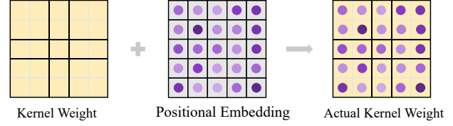
Figure 3. Illustration of kernel-wise positional embedding. The position embedding enables the kernel to distinguish specific positions in the sharing region, making up the detail-capturing ability of large kernels.
