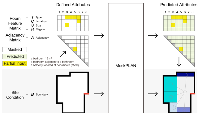
Figure 1. MaskPLAN allows users to influence layout generation with just the features they prioritize, using partial inputs in a Graph-structured Dynamic Masked Autoencoder (GDMAE) equipped with five attribute-specific generative transformers for predicting layouts from incomplete design ideas.
