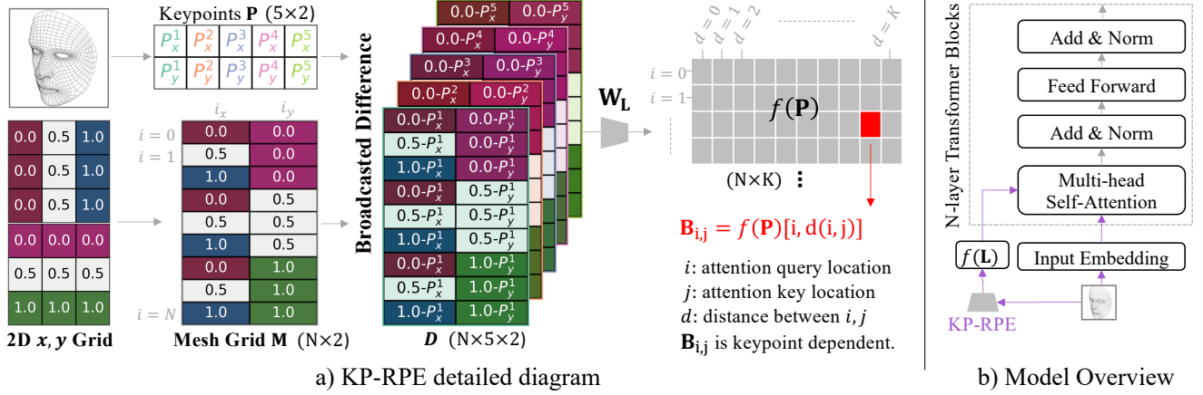
Figure 4. a) Illustration of KP-RPE. First a mesh grid M and an image-specific keypoints P are generated. Then the broadcasted difference D is calculated, and we linearly map D to f(P) . Finally for a given i, j , we can find the B_{ij} = f(P)[i, d(i, j)] , which is used to adjust the attention map in self-attention. b) Backbone contains multiple transformer blocks followed by an MLP for classification. KP-RPE is used where multi-head attention modules exist. KP-RPE is efficient as f(P) is computed once.
