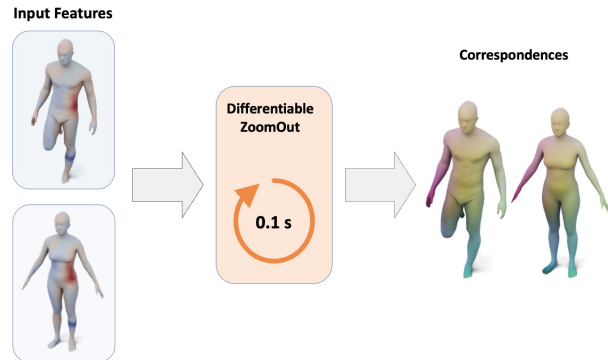
Figure 1. Our method takes a set of point features as input, which can be learned, and uses a differentiable version of the ZoomOut algorithm to produce correspondences. Due to its light memory cost, it can be used while training a network, or when running the network on very dense meshes.
