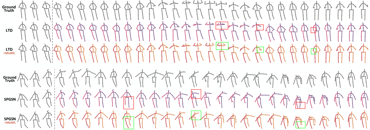
Figure 4. Two visualized cases on discussion (top) and walking dog (bottom). We choose LTD [30] and SPGSN [26] as baselines for comparison. In each case, we draw motion contents in eight seconds. With the online adaptation operation by MoML, we can produce predictions with higher accuracy, indicated by the improved performance marked in green boxes.
