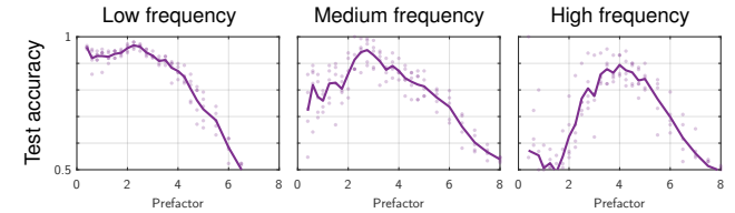
Figure 8. Detail of Figure 7 for Gaussian activations. The peak accuracy shifts to the right on tasks of increasing complexity. This corresponds to a larger prefactor that shifts the bias towards higher complexity. Each point represents one random seed.
