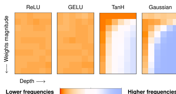
Figure 1. We examine the complexity of the functions implemented by various MLP architectures. We find that much of their generalization capabilities can be understood independently from the optimization, training objective, scaling, or even data distribution. For example, ReLU and GELU networks (left) overwhelmingly represent low-frequency functions for any network depth or weight magnitude . Other activations lack this property.
