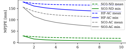
Figure 4. Minimum MPJPE and MPJPE of the mean pose for HuProSO3, ancestor-conditioned SO(3), and HF-AC for randomly occluded joints ( p_m = 0.3 ) with varying numbers of samples.
