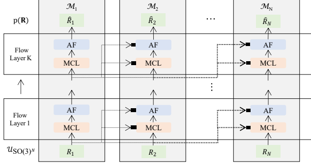
Figure 2. Overview of the components of the normalizing flow: The flow is defined on a product space of N manifolds \mathcal{M}_i = \text{SO}(3) . It includes K flow layers that transform samples R_i from a uniform distribution on \text{SO}(3) to samples of the learned distribution \hat{R}_j . The flow is composed of a Möbius coupling layer (MCL) and a quaternion affine transformation (AF). Vertical arrows indicate the flow of \text{SO}(3) samples through layers, while dotted arrows represent autoregressive conditioning using an MLP (black boxes).
