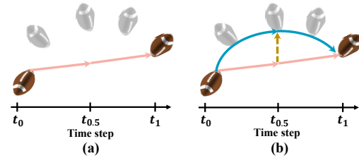
Figure 1. (a) linear methods: synthesizing the intermediate frame by fitting the linearly approximate intermediate flow (see orange trajectory). (b) our method: exploring latent acceleration prior (see yellow dotted line) to promote (a), which can model the complex scenario, like curvilinear motion (see dark green trajectory).
