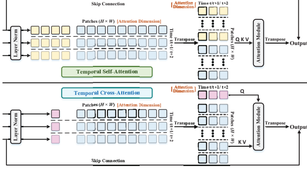
Figure 4. Illustration of the Temporal Self/Cross-Attention. For self-attention, patch embeddings of the template and search region are jointly modeled on the temporal dimension. In contrast, the cross-attention takes target queries as Q and patch embeddings of search region as K, V to extract localization-relevant information.
