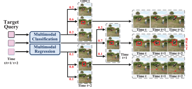
Figure 5. Illustration of the Multimodal Prediction. The target queries of different timestamps respectively predict the probabilities and locations of three possible future situations, in which the one of the highest probability score is the final output.
