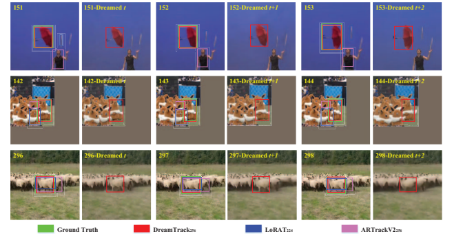
Figure 7. Results visualization of different trackers and dreamed future frames based on learned environmental dynamics.
