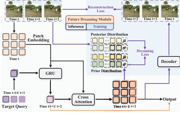
Figure 3. Illustration of the proposed Future Dreaming module. The target queries auto-regressively update the temporal dynamics with the patch embeddings of the current frame through GRU, which are then exploited to predict the future states. For training, the distributions of the predicted future states and decoded future images are self-supervised by the ground-truth future frames.
