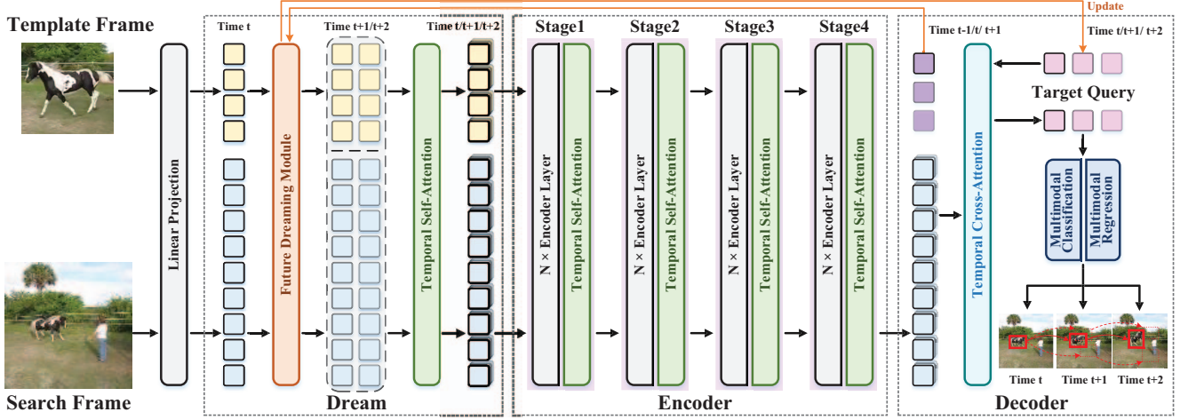
Figure 2. The dream-encoder-decoder framework of our DreamTrack. Initially, the dreaming stage takes the input image tokens to predict future states of the next two frames based on the cached temporal dynamics in the Future Dreaming module. Then features of the current frame and dreamed future are fed into the encoder for further modeling, with a Temporal Self-Attention after each encoder stage for target-aware refinement. In the end, the decoder performs multimodal prediction for the target, i.e. , the probabilities and trajectories in the current and next two frames of three possible future scenarios. The prediction with the highest probability is selected as the final output.
