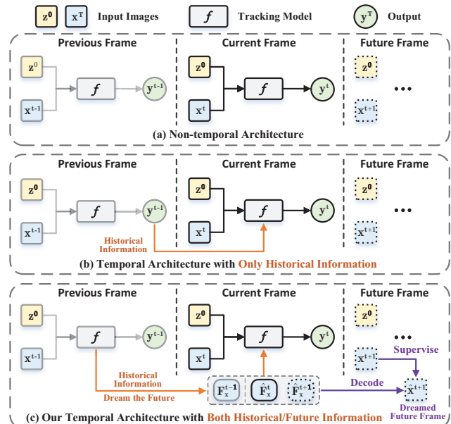
Figure 1. Comparison of different temporal architectures. (a) The non-temporal architecture that regards visual tracking as a one-shot detection problem. (b) The temporal architecture with only historical information that limits the temporal messages in the transmission of previous observations. (c) Our proposed temporal architecture with both historical and future information, which learns environmental dynamics from past experiences and dreams the future states for better generalization in subsequent frames.
