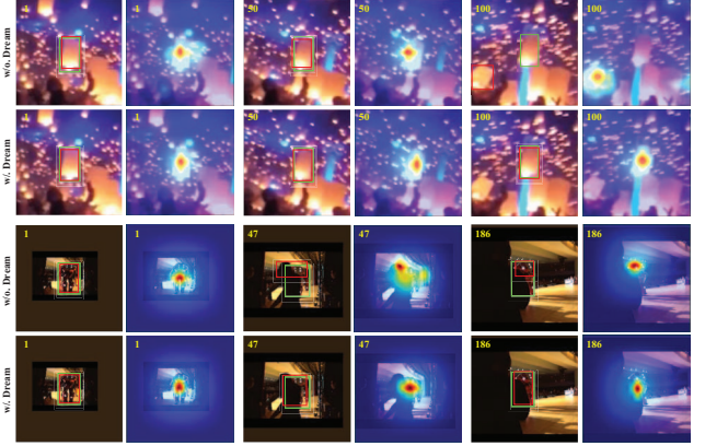
Figure 6. Attention visualization of our DreamTrack w/. and w/o. the Future Dreaming module. The predictions and ground-truth boxes are marked in red and green, respectively.
