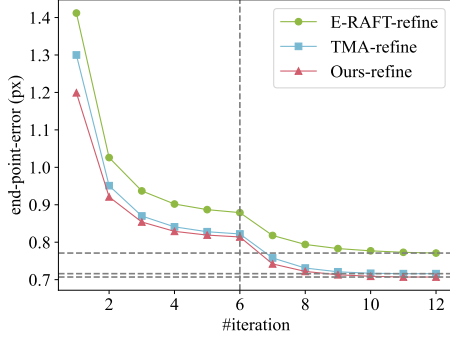
(a) EPE vs. iteration at inference. The addition of refinement stages (starting from iteration=7) results in a notable improvement in accuracy.
