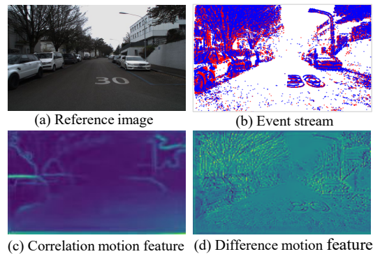
Figure 1. Illustration of difference between correlation and difference motion features. (a) Reference image of DSEC [11] dataset. (b) Corresponding event stream. (c) Correlation motion feature. (d) Difference motion feature.
