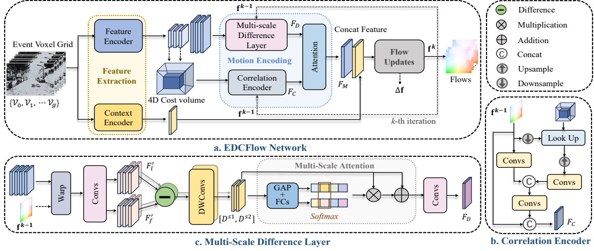
Figure 2. a. Overview of EDCFlow , including three main components: 1) Feature Extraction . Feature and context encoder extract features from input. 2) Motion Encoding . A correlation encoder and multi-scale temporal feature difference layer, along with an attention layer, are utilized to iteratively generate representative motion features. 3) Flow Updates . A GRU recurrently updates the flow by decoding the fused motion feature. b. Correlation Encoder . Search correlations at lower resolution, followed by upsampling and high-resolution correlation motion encoding. c. Multi-scale Difference Layer . Compute temporal multi-scale difference motion features at the higher resolution.
