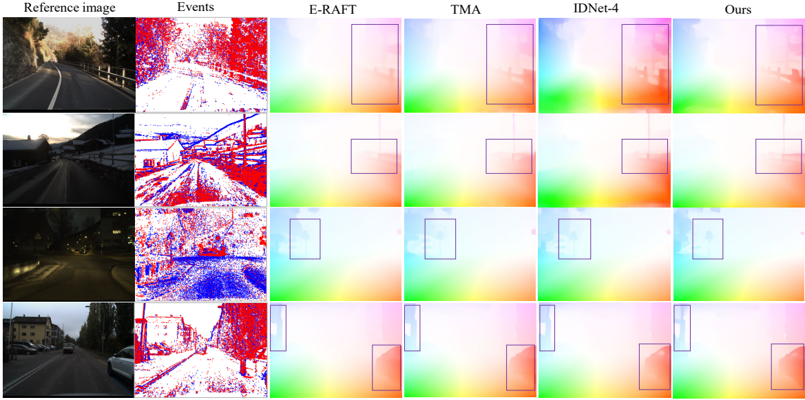
Figure 3. Qualitative results of flow predictions on DSEC [11]. Notable areas are marked by bounding boxes. Please zoom in for details.
