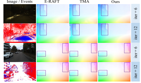
(b) Qualitative results. For each sample, we present the results before refinement (iter=6) and the final flow after refinement (iter=12).
