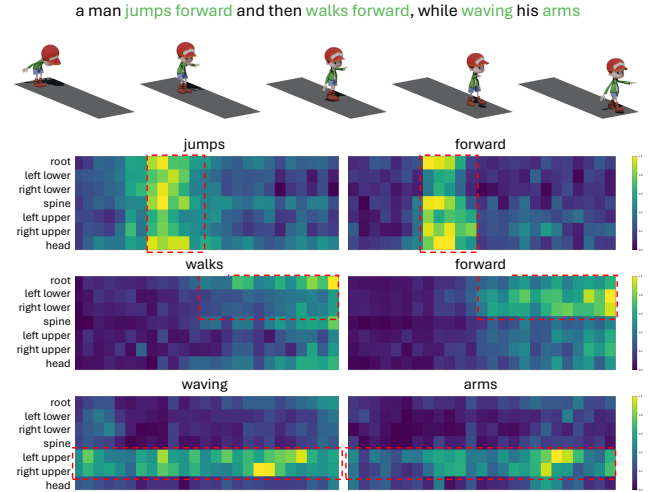
Figure 6. Visualizations of cross-attention maps of SALAD. Each row corresponds to a specific body part, and each column represents temporal frames. Attention maps were computed by averaging the output attention maps across all transformer layers and all diffusion timesteps.
