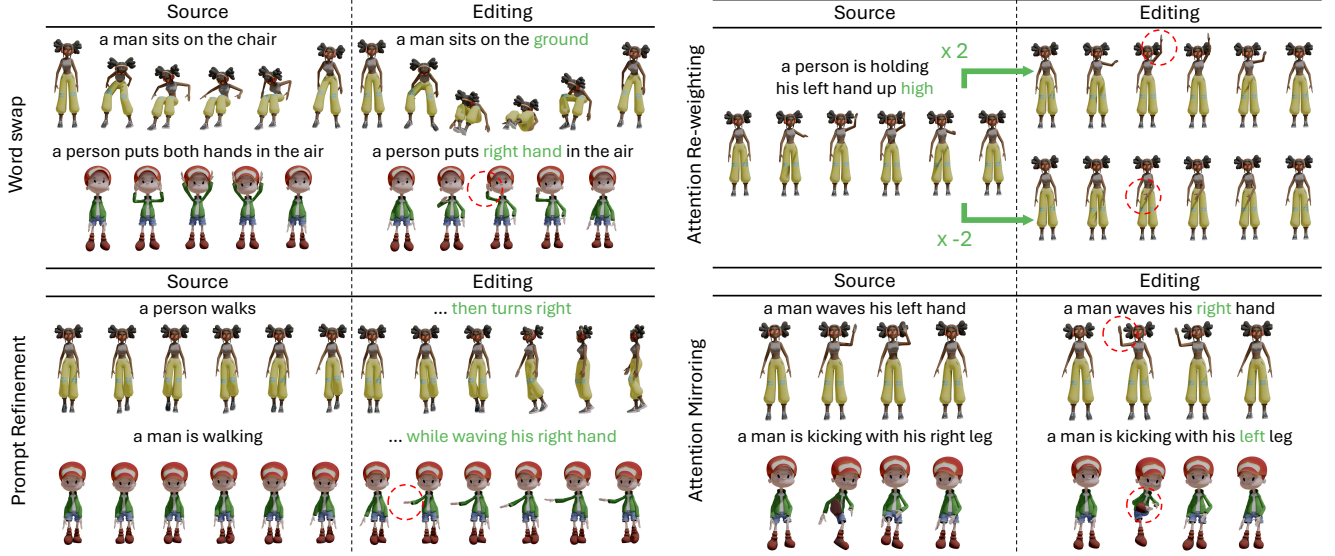
Figure 7. Text-driven motion editing results via attention modulation using a pre-trained SALAD model. Texts colored in green represent the editing instructions.
