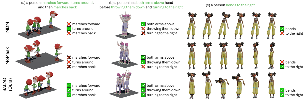
Figure 4. Qualitative comparison of results generated by various methods, including MDM [42], MoMask [12], and our approach.
