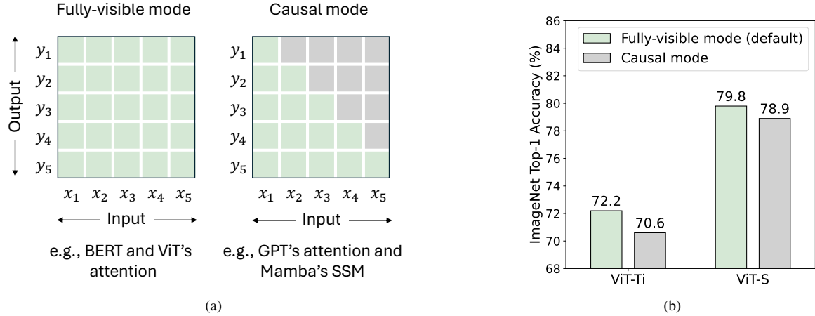
Figure 3. (a) Two modes of token mixing [69]. For a total of T tokens, the fully-visible mode allows token t to aggregate inputs from all tokens, i.e., \{x_i\}_{i=1}^T , to compute its output y_t . In contrast, the causal mode restricts token t to only aggregate inputs from preceding and current tokens \{x_i\}_{i=1}^t . By default, attention operates in fully-visible mode but can be adjusted to causal mode with causal attention masks. RNN-like models, such as Mamba’s SSM [28, 29], inherently operate in causal mode due to their recurrent nature. (b) We modify the ViT’s attention [26, 79] from fully-visible to causal mode and observe performance drop on ImageNet, which indicates causal mixing is unnecessary for understanding tasks.
