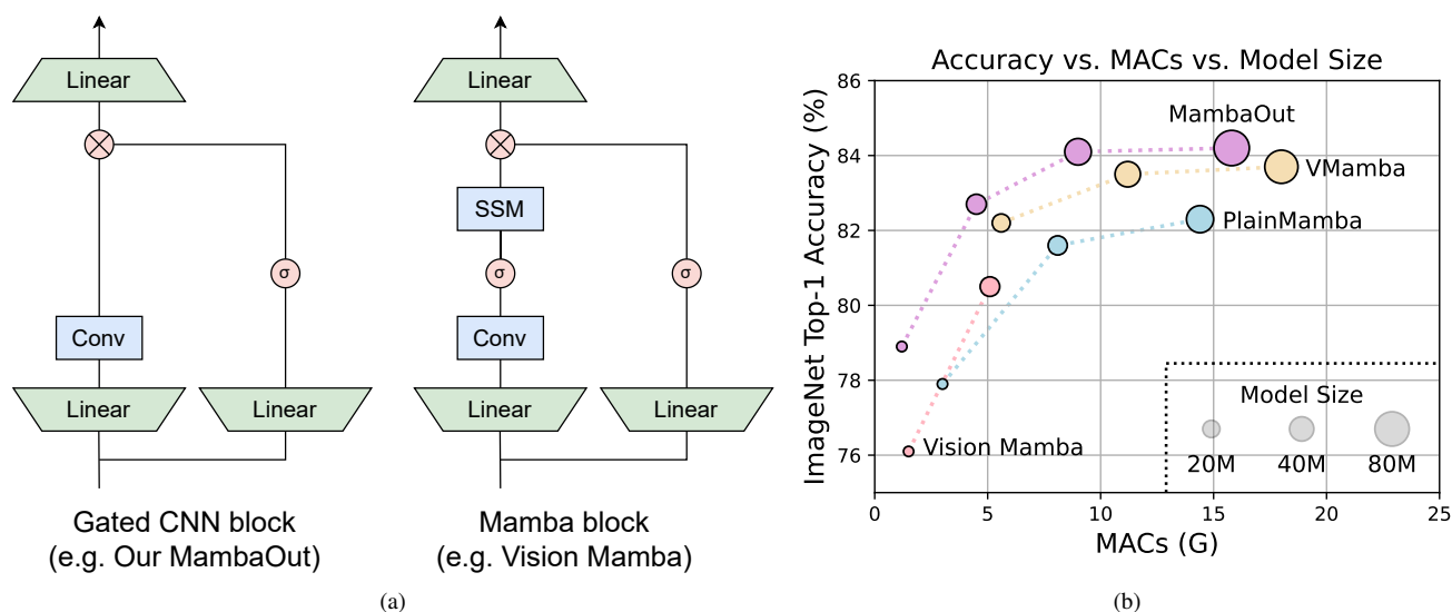
Figure 1. (a) Architecture of Gated CNN [20] and Mamba [28] blocks (omitting Normalization and shortcut). The Mamba block extends the Gated CNN with an additional state space model (SSM). As will be conceptually discussed in Section 3, SSM is not necessary for image classification on ImageNet [21, 72]. To empirically verify this claim, we stack Gated CNN blocks to build a series of models named MambaOut . (b) MambaOut outperforms visual Mamba models, e.g., Vision Mamba [112], VMamba [56] and PlainMamba [96], on ImageNet image classification.
