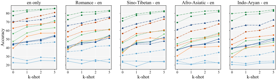
(c) CM-TruthfulQA
