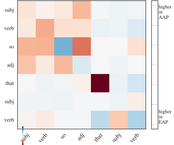
Figure 12: This plot shows which interactions, on average , most substantially differ between EAP and AAP examples. From highest to lowest in absolute value we have that with itself, so with adj , so with itself, verb with itself, and so with verb .
