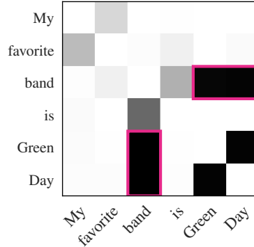
Figure 9: The local affinity matrix reflects interactions (pink) between band , Green , and Day , as expected.
