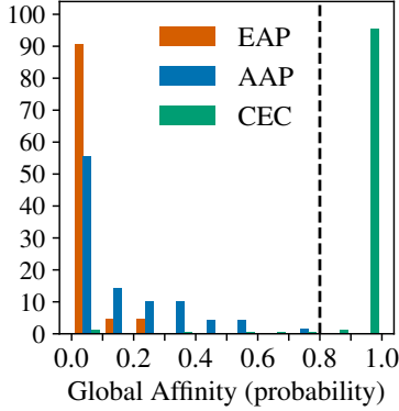
Figure 2: Percent of examples with so having given global affinity. The CEC is seen to be well-separated from the EAP and AAP.
