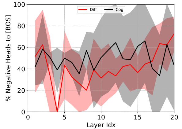
Figure 5: Percentage of attention head scores with negative values from all tokens in the sequence that point to the [BOS] token. These scores are computed for all layers of the COG and DIFF 125M scale Transformer models. The curve represents the mean, and the shaded area indicates the standard deviation across all attention heads.
