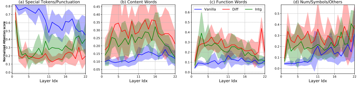
Figure 3: Normalized attention scores of continuation tokens (see Appendix A.4) attending to all tokens in the sequence, grouped into four token types. These scores are computed for all layers of the VANILLA, DIFF, and INTG 1.2B-scale Transformer models. The curve represents the mean, and the shaded area indicates the standard deviation across all attention heads.
