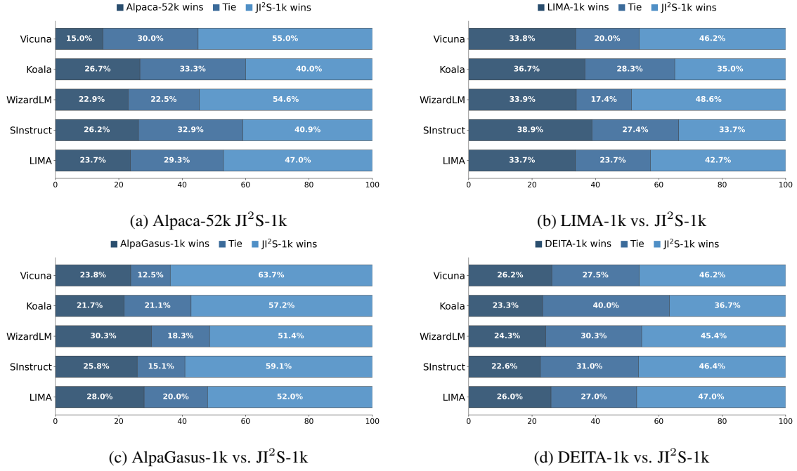
Figure 3: GPT-4-judged win rates of JI²S-1k versus four baselines (Alpaca-52k, LIMA-1k, AlpagaGasus-1k, DEITA-1k) across five evaluation datasets.
