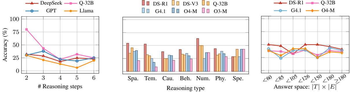
(a) Average accuracy among each model family declines as the number of annotated reasoning steps increases. (b) Accuracy with respect to the reasoning types. While performance vary a lot across models, causal reasoning is usually the weakest. (c) Accuracy with respect to size of answer space. Results does not show strong negative correlation.
