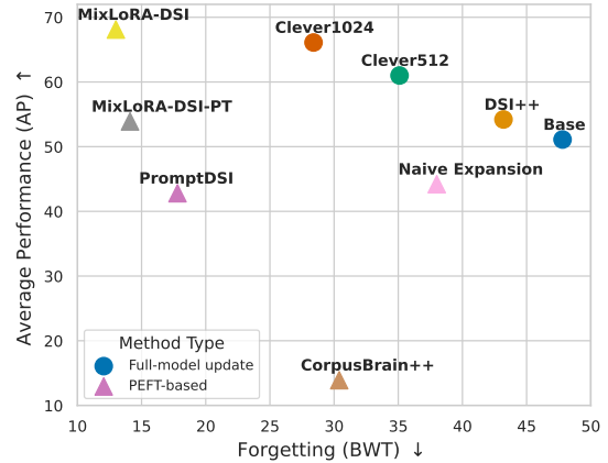
Figure 1: Continual learning performance of different Generative Retrieval methods on NQ320k (Recall@10). PEFT-based MixLoRA-DSI variants offer the best trade-off between average performance and forgetting, while being significantly more parameter-efficient than full-model updates. See Table 1 for more detailed results.
