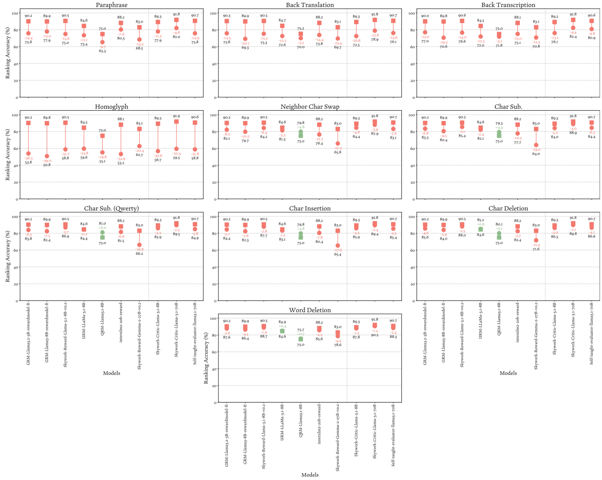
Figure 6: The change of RM ranking accuracy under meaning- or ranking-preserving (natural) reWordBench transformations.
