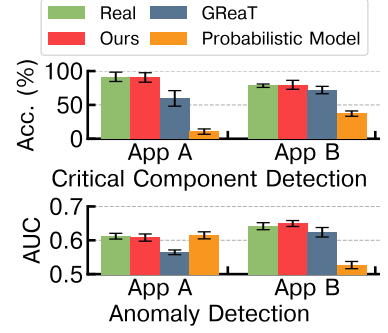
Figure 5: ML Model Performance (real vs. synthetic traces).
