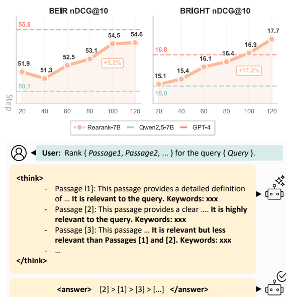
Figure 1: (Top) Average rerank results on popular benchmarks (over BM25 top 100), the performance improves with RL training; (Bottom) REARANK inference example. The agent provides the reasoning and final ranking of all passages, unlike current agents (Sun et al., 2023; Pradeep et al., 2023b) that only output the final answer.
