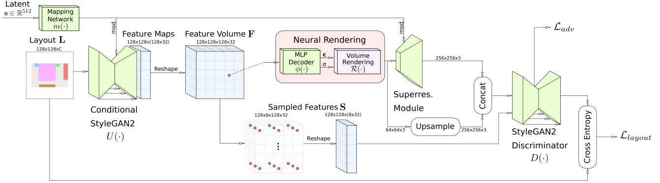
Figure 3. Architecture – Our method takes a floorplan projection of the semantic scene layout and a noise vector as inputs. We use a conditional StyleGAN2 backbone to generate a 2D feature field based on the given layout and reshape the channels into a 3D feature volume. This feature volume is queried using trilinear interpolation and subsequently decoded into color and density using a small MLP. We use a superresolution module to upsample volume rendered images to target resolution and use a standard StyleGAN2 discriminator. In order to ensure semantic consistency between the layout and the rendering, we sample equidistant coordinates from the feature volume and process the sampled features with a semantic segmentation decoder added to the discriminator. We train our model on a combination of an adversarial loss and cross entropy loss.
