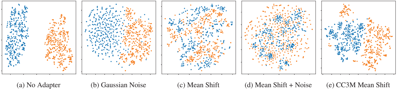
Figure 3: t-SNE [64] plots for various adapters on 350 randomly selected image vectors (blue) and paired caption vectors (orange) from COCO captions. The first two panels demonstrate CLOSE, and the remaining three show additional adapters we study in our analysis (Section 4).
