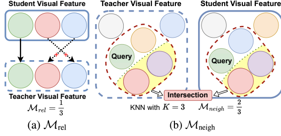
Figure 2: Illustrations of \mathcal{M}_{\text{rel}} and \mathcal{M}_{\text{neigh}} that measure the coherence of relative visual feature relationship and local visual space structure between the student and teacher. Each color corresponds to a single image. In (a), arrows indicate the nearest neighbors from student’s visual space to teacher’s visual space. Solid lines represent correct matching, while dashed lines indicate incorrect matching. In (b), the green circle represents a query image, and the red dashed regions represent the k -nearest neighbors (kNN) in both spaces. We measure the intersection between the two kNN sets.
