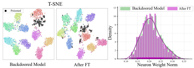
Figure 1: Left: T-SNE [45] visualization on the backdoored model and the model after fine-tuning. FT fails to remove backdoor effect. Right: the neuron weight norm distribution between the two models. The weight seems to have remained mostly unchanged after the fine-tuning process.
