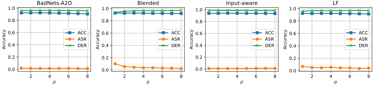
Figure 3: Performance of FT-SAM with \rho from 1 to 8 against attacks on CIFAR-10 and 10% poisoning ratio with PreAct-ResNet18.
