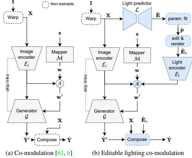
Figure 3. Overview of our proposed editable lighting co-modulation method. The input image I is first warped according to its (known) camera parameters to a 360^\circ panorama X via a (non-trainable) warp. (a) As proposed in [61, 6], an image encoder \mathcal{E}_i co-modulates (with the mapper \mathcal{M} ) the generator network \mathcal{G} according to X . Here, A denotes a (learnable) affine transformation. (b) Our editable light co-modulation method first estimates an HDR light map \hat{E} from the warped image X through a light predictor \mathcal{L} . The light map is converted to a parametric model \hat{p} and can optionally be edited by a user to obtain \hat{p}_e before being re-rendered to an image \hat{E}_e and injected in the style co-modulation mechanism via a light encoder \mathcal{E}_l . Our proposed novel components are highlighted in blue.
