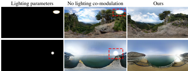
Figure 8. Ablation study on the effect of our proposed lighting co-modulation. Using the lighting co-modulation helps blending realistically the lighting parameters into the surrounding.
