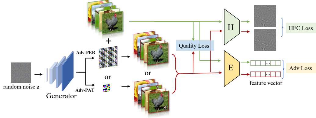
Figure 3: The pipeline of our attack
