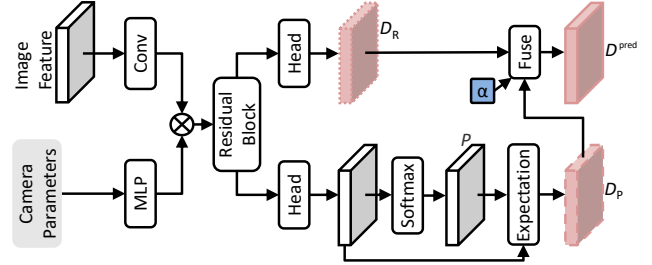
Figure 4. Framework for depth head. The depth estimation D^{pred} is the fusion result of regressed depth D^R and probabilistic depth D^P , \alpha is the fusion weight, P is the probabilistic over depth bins.
