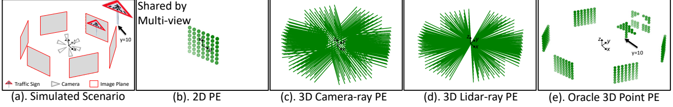
Figure 2. Illustration of different positional encoding in the surround-view system. (a) presents the simulated scenario with 6 cameras, only one traffic sign appears in front view (the distance is set as 10m), rather than other cameras. Comparing all the PE from (b) to (e), only the oracle 3D point PE can encode the precise 3D point location of the object. Best viewed in color.
