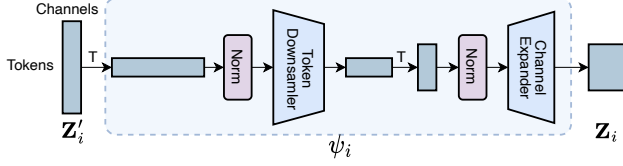
Figure 4: Token mixer . The token downsampler performs per-channel interaction along the token dimension, and the channel expander performs per-token interaction along the channel dimension. The operations in the light blue block ( \psi_i ) correspond to a blue arrow in Fig. 2.
