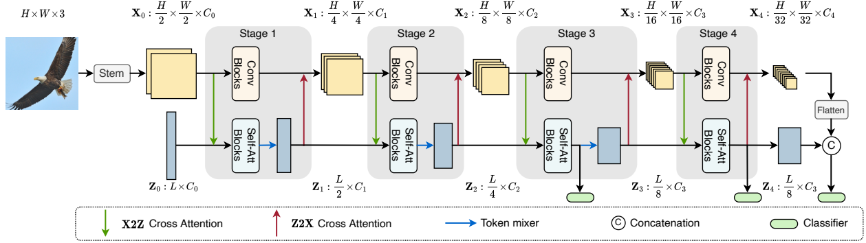
Figure 2: An overview of Dyn-Perceiver. The feature branch (top) and the classification branch (bottom) process image features X_0, \dots, X_4 and the latent code Z_0, \dots, Z_4 respectively. Cross-attention layers are built symmetrically to fuse information from the two branches. Early classifiers are appended only in the classification branch. Best viewed in color.
