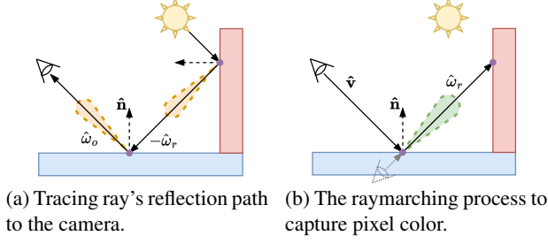
Figure 6: The illustrations of inter-reflections from the (a) physical lighting process and (b) raymarching rendering process. We assume the surface has a low roughness value.
