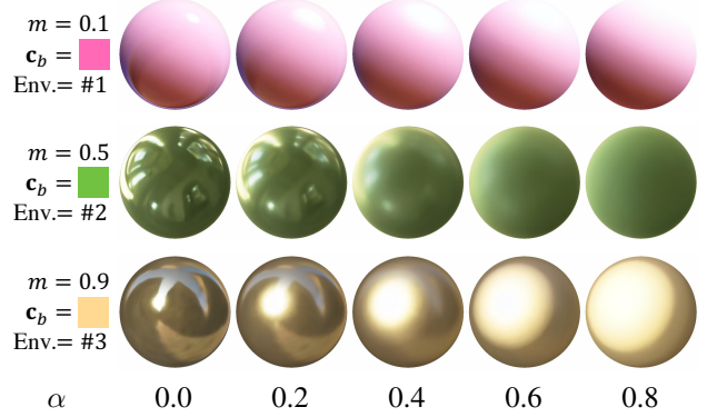
Figure 5: Spheres synthesized by our neural renderer with varying metallic m , base color \mathbf{c}_b , roughness \alpha , and light probes. We will show an interactive web demo in the future.
