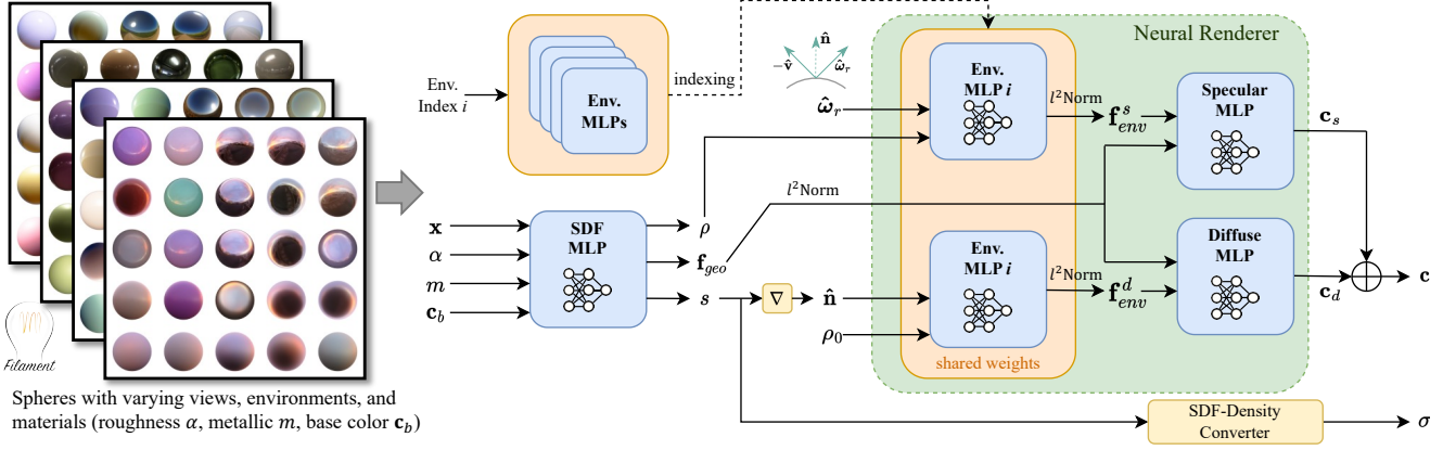
Figure 3: Overview of our proposed neural renderer. Training images are synthesized by Filament PBR engine [29] during runtime, and probes are from HDRI Haven (CC-0). The MLPs in our neural renderer are some simple and tiny MLPs.
