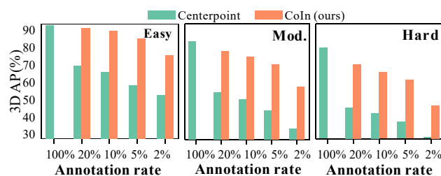
Figure 1. Comparison of performance with different annotation rates under the KITTI-3D-Car. Green and orange represent CenterPoint[39] and our proposed CoIn, respectively.
