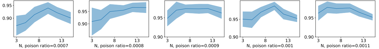
Figure 9. ASR of the RD score in different poison ratios when the iteration time N in greedy search changes. We repeat each experiment three times. In all the experiments, we set the training epoch of the scoring model to 6
