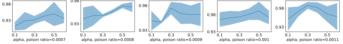
Figure 8. ASR of the RD score in different poison ratios when \alpha in greedy search changes. We repeat each experiment three times. In all the experiments, we set N to 10 and the training epoch of the scoring model to 6
