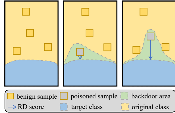
Figure 1. Intuitive explanation of our insight. The left figure shows a clean model without any backdoor. In the middle figure, a sample closer to the decision boundary will have less impact on the backdoor when it is poisoned. In the right figure, a sample farther away from the decision boundary can cause a more significant change to the model when it is selected for poisoning.
