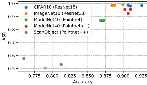
Figure 7. ASR and prediction accuracy on various models and tasks. All the ASRs are obtained using RD scores at the highest poison ratio we use in the experiments, i.e., 0.0017 for CIFAR-10, 0.0095 for ImageNet-10, 0.01 for ModelNet40, and 0.09 for ScanObject. At the above ratios, the ASR of the backdoors becomes stable.
