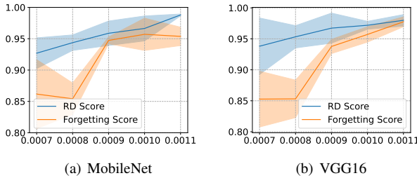
Figure 11. ASRs of the forgetting score and our RD score. We use ResNet18 as the victim model and change the architecture of the scoring model to MobileNet and VGG16.
