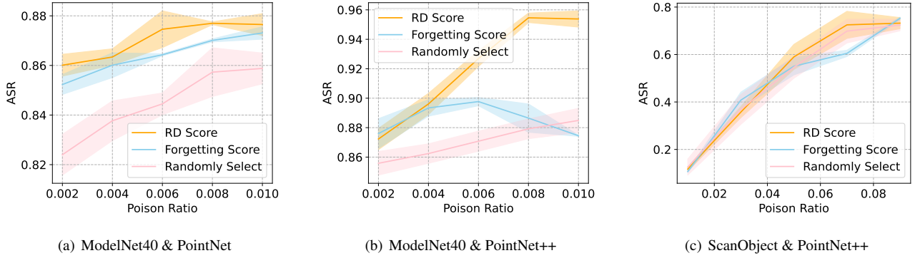
Figure 6. ASR of the three methods on 3D point cloud classification tasks. We repeat the experiments three times for the scoring-based methods and 5 times for random selection. We reduce the iteration time N to 7 when conducting the greedy search on both of the scoring methods. For ScanObject, we set the training epoch to 75 and the learning rate to 0.01.
