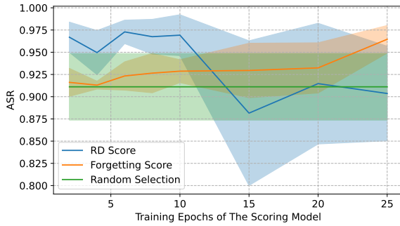
Figure 10. The influence of the training epoch of the scoring models on both methods. All the experiments are conducted using a 0.001 poison ratio on CIFAR-10, ResNet18.
