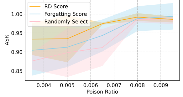
Figure 5. ASR of the three methods on ImageNet-10. We repeat the experiments three times for both score-based selection strategies and five times for random selection. We set \alpha to 0.3 and N to 10. The training epoch of the models for RD score is 6 while that for forgetting score is 30.
