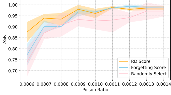
Figure 4. ASR of the three methods on CIFAR-10. We repeat the experiments three times for both score-based selection strategies and ten times for random selection. We set \alpha to 0.3 and N to 10. The training epoch of the models for RD score is 6 while that for forgetting score is 50.
