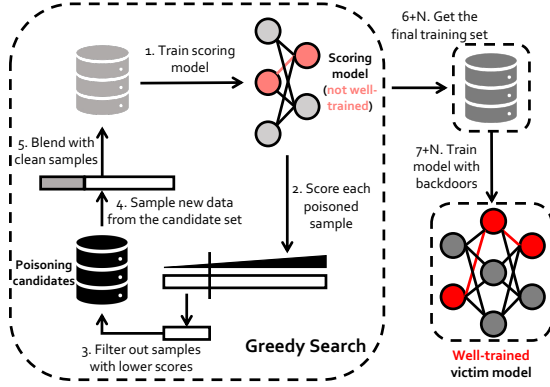
Figure 2. Workflow of our methodology.
