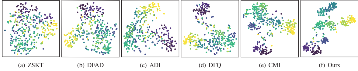
Figure 5. Visualization of t-SNE distribution on Aircraft dataset.
