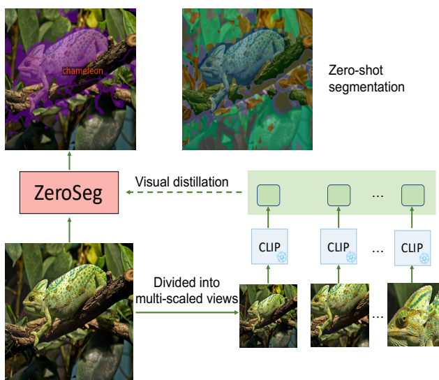
Figure 1. ZeroSeg overview. ZeroSeg is a zero-shot open-vocabulary method for semantic segmentation. The approach begins by dividing the input image into a set of multi-scale views. Each view is then individually processed by a pretrained CLIP visual encoder model to extract visual concepts. These visual concepts are then distilled into our ZeroSeg model via the proposed segment matching loss. After training, our ZeroSeg model can be directly transferred to downstream semantic segmentation tasks in a zero-shot manner ( i.e. , no training or adaption on target datasets).
