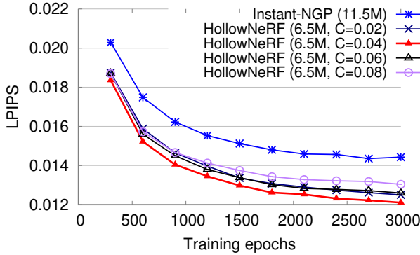
(b) LPIPS \downarrow (lower is better).
