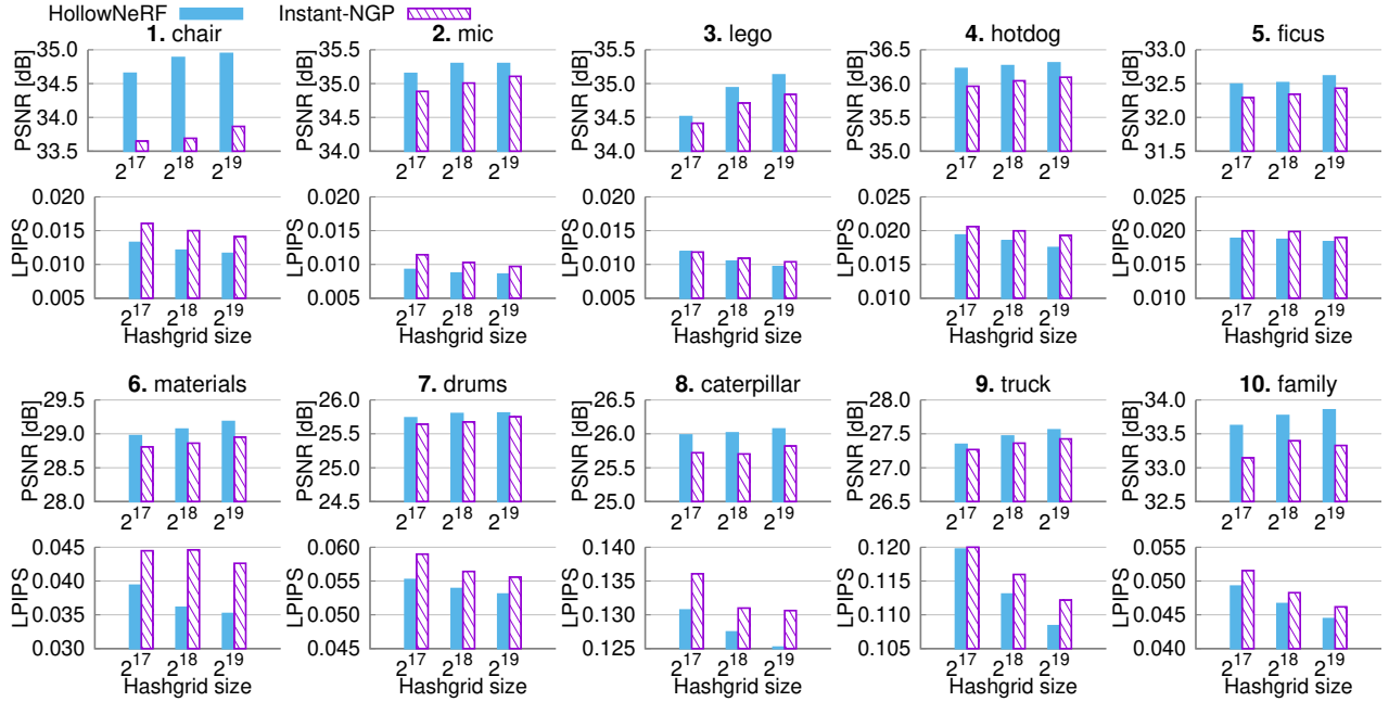
Figure 8: Comparison of PSNR(↑) and LPIPS(↓) performance between HollowNeRF and Instant-NGP on various scenes.
