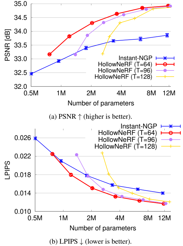
Figure 4: Performance vs. saliency grid size T .
