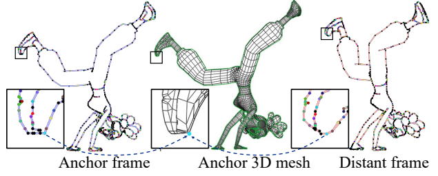
Figure 3: Geometrized line art in MixamoLine240 . 2D endpoints and connected lines are projected from vertices and edges of orinal 3D mesh. Endpoints indexed to unique 3D vertices are matched (marked in the same colors).
