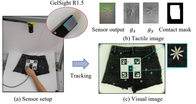
Figure 3: Visual-tactile data acquisition setup. (a) Our setup includes a PiCamera RGB camera, a GelSight R1.5 high-resolution tactile sensor, and Aruco markers to track the relative pose of the sensor. (b) We show the captured tactile data, including the raw sensor output, the derived surface gradients in x and y directions g_x and g_y , and the computed contact mask. (c) We locate the bounding box in the visual image corresponding to the tactile data.
