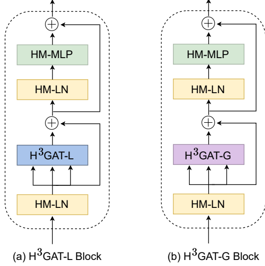
Figure 5: Transformer blocks for local and global attentions.
