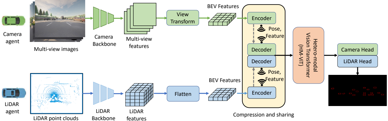
Figure 3: Overview of proposed hetero-modal V2V cooperative perception system. Each agent first produces BEV features through modality-specific feature extractors (Sec. 3.1). The BEV features are then compressed and shared (Sec. 3.3) with neighboring connected agents and the received features are decompressed in the ego agent side and fed into hetero-modal vision transformer to conduct graph-structured feature fusion (Sec. 3.2 and Sec. 3.3). The refined features are finally passed into the hetero-modal detection head to predict 3D bounding boxes (Sec. 3.4).
