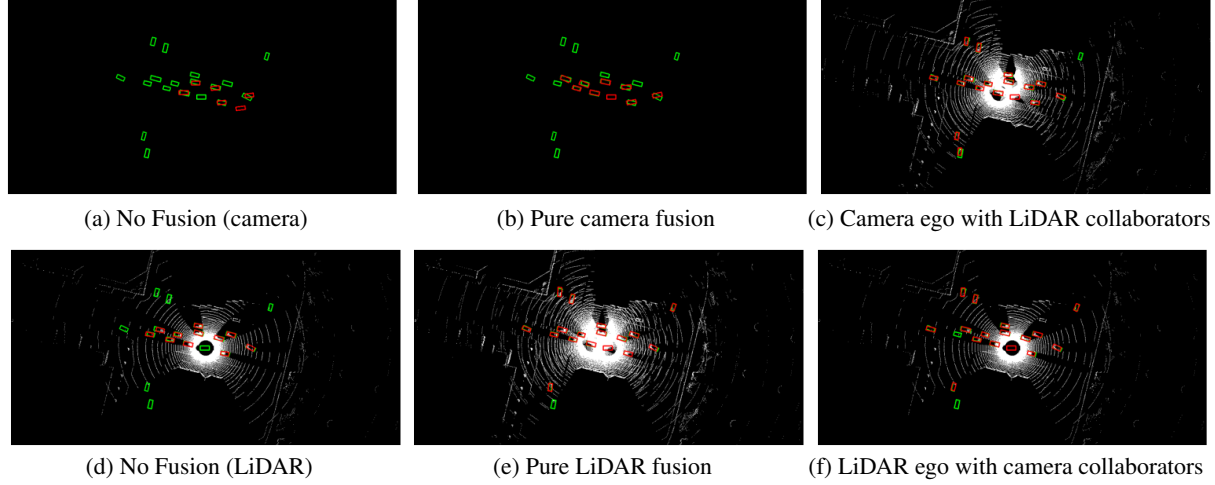
Figure 8: Qualitative visualizations for (a) No Fusion with camera ego vehicle, (b) pure camera-based V2V perception, (c) hetero-modal V2V perception with camera ego vehicle and LiDAR collaborators, (d) No Fusion with LiDAR ego vehicle, (e) pure LiDAR-based V2V perception, and (f) hetero-modal V2V perception with LiDAR ego vehicle and camera collaborators. The red and green boxes represent the detection outputs and ground truth respectively. More visualizations can be found in the supplementary materials.
