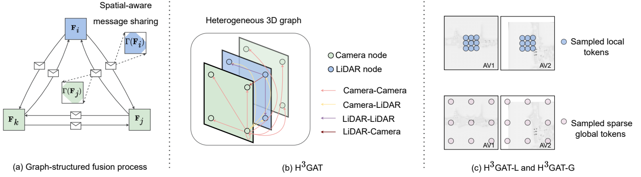
Figure 4: HM-ViT architecture. (a) Graph-structured fusion process. (b) Heterogeneous 3D graph attention ( H^3GAT ). (c) Illustration of sampled tokens for H^3GAT-L and H^3GAT-G .
