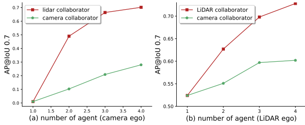
Figure 7: Ablation study on number of agent. The LiDAR/camera collaborator refers to the case where the collaborators are equipped with LiDAR and Camera respectively. (a) ego vehicle is equipped with camera. (b) ego vehicle is equipped with LiDAR.
