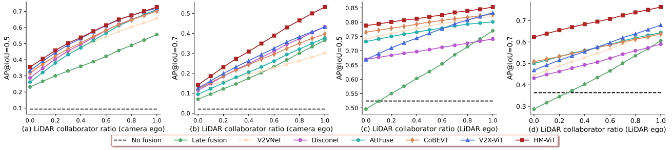
Figure 6: Agent modality ratio experiment. The x-axis is the ratio of LiDAR collaborators among all the collaborators. In (a) and (b), ego vehicles are equipped with cameras. In (c) and (d), ego vehicles are equipped with LiDARs.
