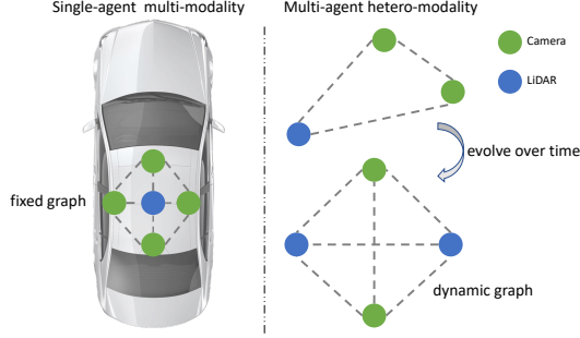
Figure 2: Comparison of the single-agent multi-modal system and multi-agent hetero-modal system. The graph structure of the former is fixed whereas for the latter the graph is both dynamic and heterogeneous.
