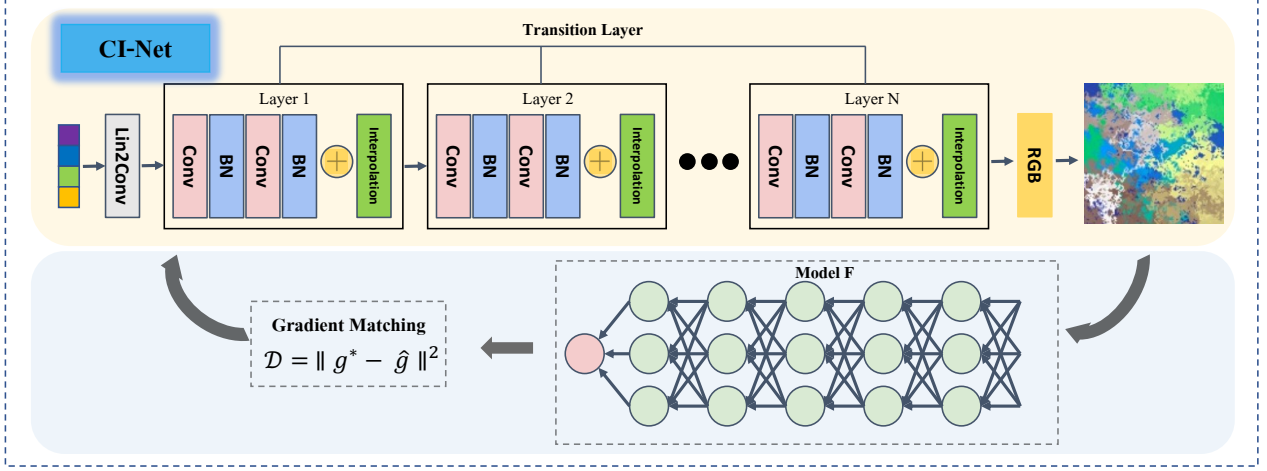
Figure 4: Architecture design of CI-Net and its model updating process.
