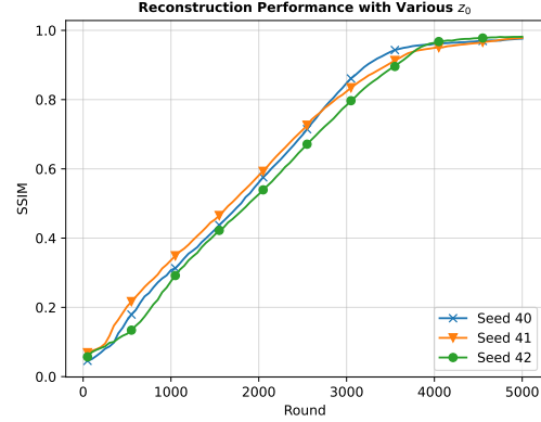
Figure 8: Image reconstruction with various z_0 .
