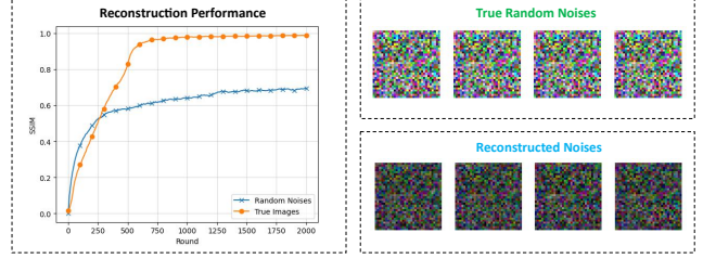
Figure 3: Ablation study on both true images and random noises. Left figure shows gradient inversion on natural images (orange line) achieves an SSIM value close to 1, while inversion of random noises (blue line) results in poor performance. The random noises and the reconstructed counterparts are plotted in the right panel, for visual comparison.
