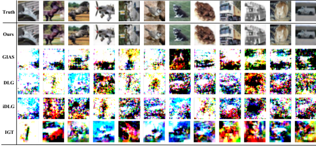
Figure 6: Sample reconstructed images on CIFAR-10 dataset, when batch size equals 128.
