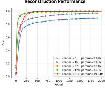
Figure 2: Ablation study on over-parameterization. P(F) \approx 0.33M . Results indicate over-parameterized models obtain an SSIM value of 1.0 for image reconstruction.
