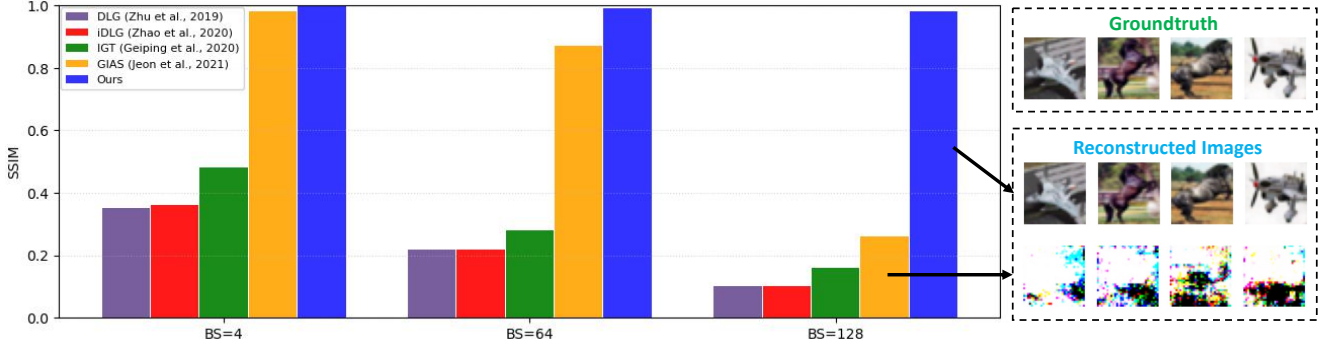
Figure 5: Gradient inversion on the CIFAR-10 dataset. The structural similarity (SSIM) noticeably decreases with an increase in batch size from 4 to 128, except for the proposed method in this paper. Additionally, four sample images from both GIAS and the proposed method are presented on the right-hand side of the figure, allowing for a visual comparison with the groundtruth.
