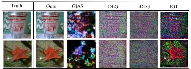
Figure 7: Sample reconstructed images on ImageNet.
