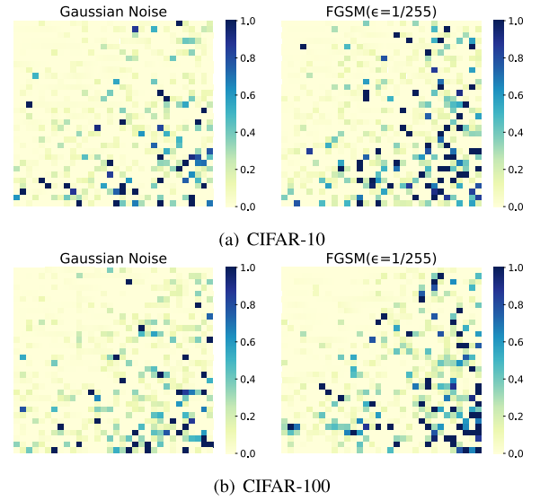
Figure 3. RCT maps for Gaussian noise and the FGSM adversarial examples [12] generated on the standard trained ResNet18. The upper left and lower right corners represent the lowest and highest frequency components in the DCT space, respectively. The deeper color indicates a greater change for a specific frequency component between the original and perturbed images, where \sigma = 0.1 for the Gaussian noise and the maximum perturbation \epsilon = 1/255 for FGSM.
