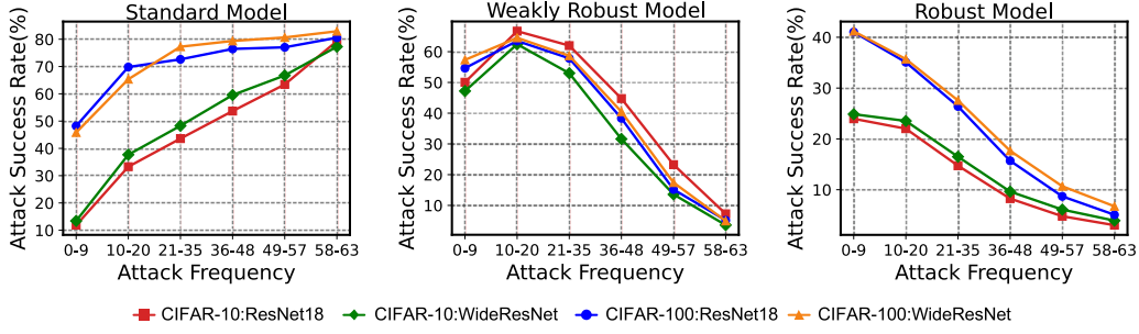
Figure 2. The attack success rate of \delta_f on different models. Standard Model is standard trained ResNet18 (WideResNet), Weakly Robust Model uses PGD attack with \epsilon = 4/255 , \alpha = 2/255 to train ResNet18 (WideResNet) for 20 epochs, and Robust Model uses PGD with \epsilon = 8/255 , \alpha = 2/255 to train ResNet18 (WideResNet) for 50 epochs.
