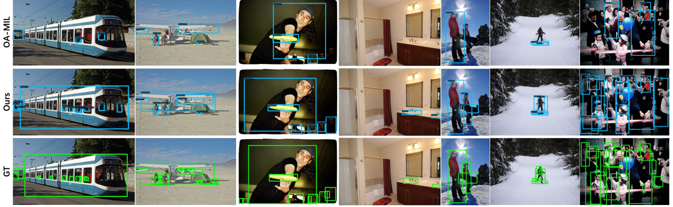
Figure 4: Qualitative detection results on COCO validation. Previous methods miss objects and face part prediction problems. Our method misses fewer objects, and the bounding box quality is better, especially for small or overlapped objects.
