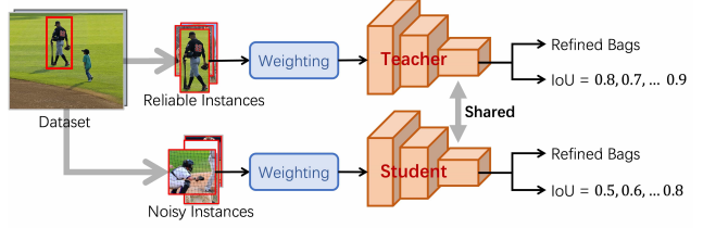
Figure 2: The mechanism of Spatial Self-Distillation. By assigning higher weight, the low-noise annotations can be seen as reliable samples to guide the training of proposals’ spatial position and identity learning in SPSP and SISD.
