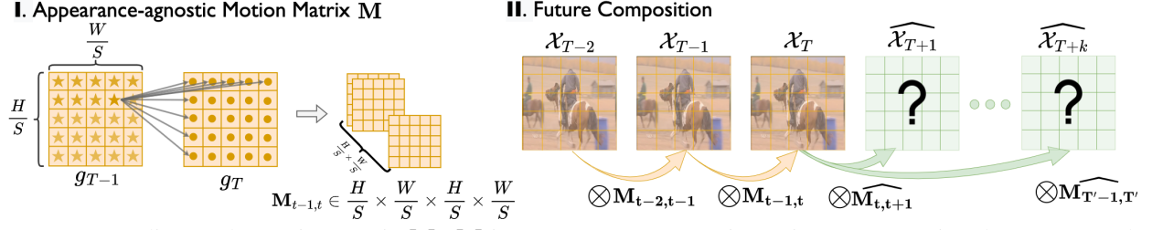
Figure 3: MMVP relies on the motion matrix \mathbf{M} . \mathbf{M} is an appearance-agnostic motion representation that measures the cosine similarity between the feature patches of two consecutive frames. Information of the past frames \{\mathcal{X}_0, \dots, \mathcal{X}_T\} can compose the future information \{\widehat{\mathcal{X}}_{T+1}, \dots, \widehat{\mathcal{X}}_{T'}\} through matrix multiplication \otimes with \mathbf{M} .
