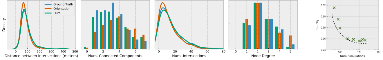
Figure 7. (Left) Comparison of generated graph statistics, following the same post-processing, averaged across regions of 400 \times 400 meters in ground distance. Orientation refers to the method of [8]. (Right) The estimated Pareto front achieved through the evaluation of various runs, where a different number of MCTS simulations is being executed at each state. obj refers to an average of the APLS , Path-based f1 , Junction-based f1 and Sub-graph-based f1 metrics.
