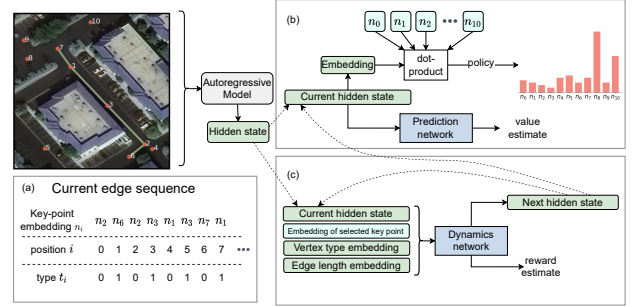
Figure 5. The autoregressive model generates a hidden state corresponding to the graph embedding. (a) When doing so, the edge decoder directly attends to the input key points’ embeddings, augmented by position and type embeddings. (b) The prediction network uses the hidden state to produce value and policy predictions. A pointer network allows an intuitive scale of the action space by the number of key points. (c) The dynamics network simulates trajectories by estimating new hidden states and rewards. For newly generated edges, it takes as input the embeddings of the new key points, but also the degree of the two vertices involved and the length of the newly proposed generated edge.
