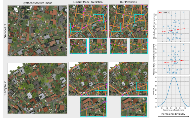
Figure 6. (Left) Examples of fragmented outputs from the LinkNet model under cases of significant occlusion and how our approach performs in these demanding circumstances. (Right) The performance gap between our method and the same baseline is wide, based on topological spatial graph metrics, for a wide range of difficulties in the images. More details and examples are given in the supplementary material.
