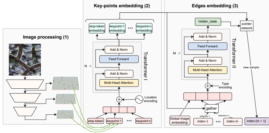
Figure 4. The autoregressive model with its three main components. (1) A backbone image model (ResNet) that extracts features for each key point at different scales, along with a global image embedding. (2) A key point model embeds visual and location features of distinct key points. (3) An edge embedding model relates the current edge sequence with the respective key points. Each edge token (signalled with the tokens ‘index- i ’) corresponds to an index specifying the respective key point. A pair of such tokens designates an edge as its two endpoints. At the end of (3) we obtain a new distribution over key points that leads to an incremental update to the graph, after sampling.
