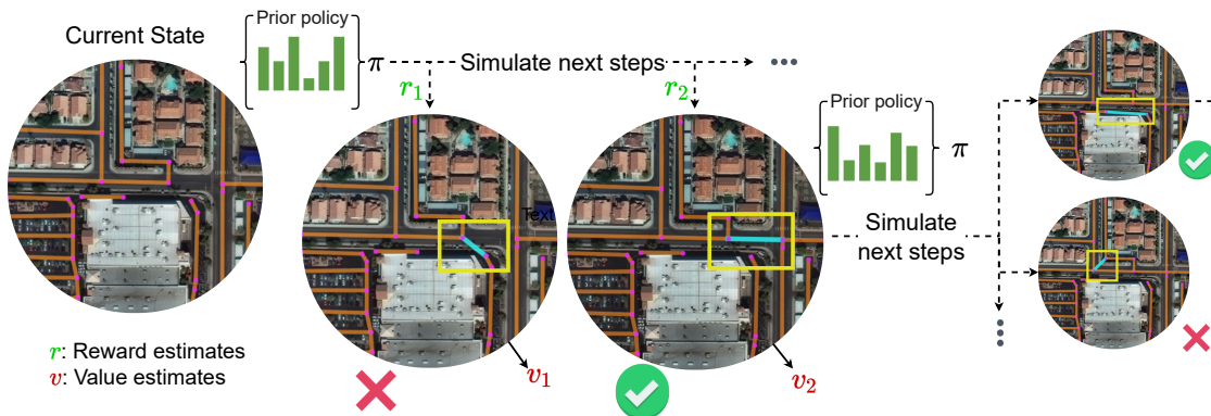
Figure 1. Our agent interacts with the currently generated spatial graph by proposing new edges to be added. A tree-based search produces a sequence of actions that maximizes a reward function based on complex geometries priors.
