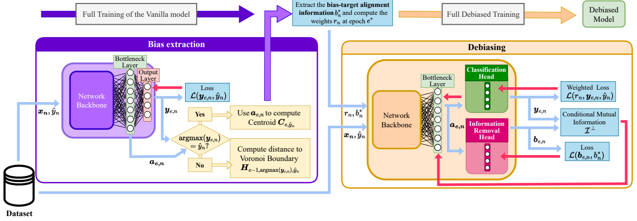
Figure 2. Overview of the proposed debiasing approach: the bias is first extracted (left) and then the unbiased model is trained (right). Blue arrows represent forward propagation while red arrows represent backpropagation.
