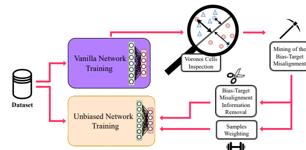
Figure 1. Our proposed approach to agnostically remove the bias.
