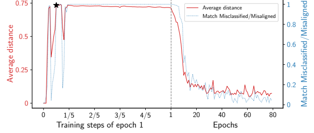
Figure 4. Evolution of the relative distance to the target Voronoi boundary for the misclassified elements (red curve) and the match between the misclassified samples \{n | \arg\max(\mathbf{y}_{e,n}) \neq \hat{y}_n\} and the misaligned samples \{n | \hat{b}_n \neq \hat{y}_n\} (blue dashed line).
