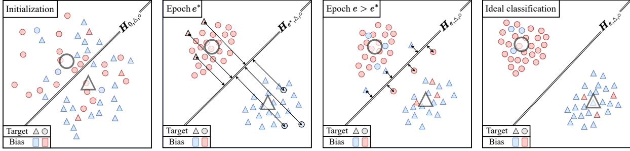
Figure 3. Representation of latent representations of a dataset at different learning stages. The target classes are shapes and the bias is color. Arrows represent the distance between misclassified elements and the Voronoi boundary.
