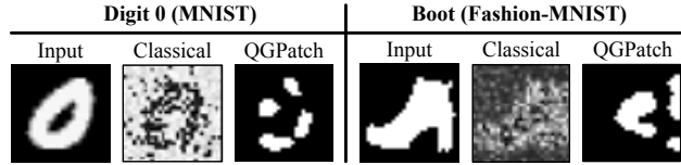
Figure 2. State-of-the-art quantum image generator, QGPatch [11], generates low-quality images for different datasets. However, its quality is still similar to a classical GAN with 25\times more parameters and iterations.
