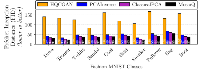
Figure 12. MosaiQ produces higher quality images on every class of the Fashion MNIST dataset as compared to HQCGAN [19] in addition to the classical methods tested.
